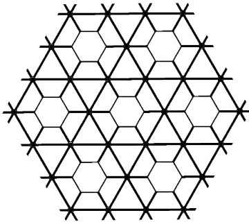
InterAx™ Foundation NXF Geogrid Plan View
