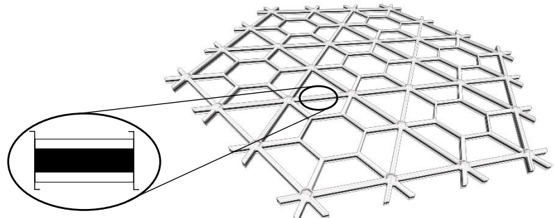
Tensor NX750 Geogrid Perspective View
