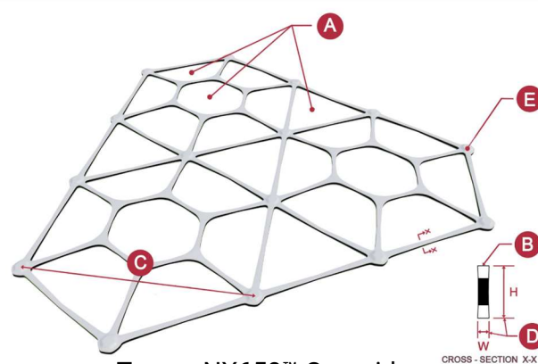
Tensar NX650™ Geogrid Plan View
