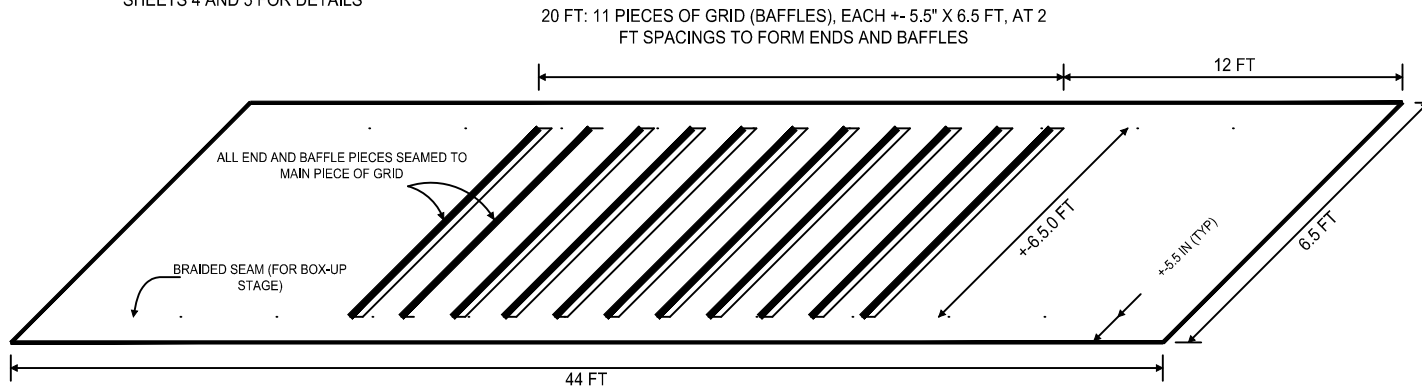
TYPICAL MARINE MATTRESS UNIT AFTER INITIAL FABRICATION
