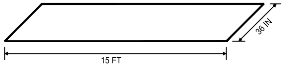
TYPICAL PRE-CUT GEOTEXTILE STRIP FOR END COMPARTMENTS
