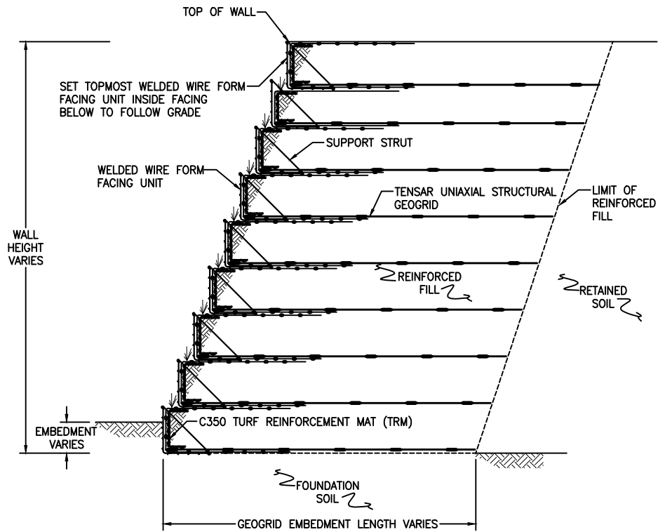
SIERRA SLOPE TYPICAL CROSS-SECTION
