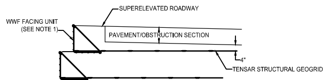
SUPERELEVATED PAVEMENT/OBSTRUCTION STRUCTURE
